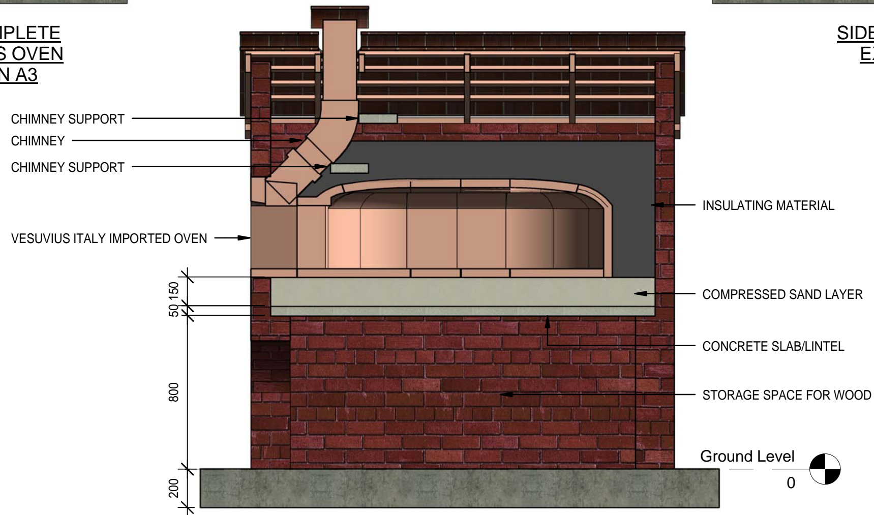
SECTION OF COMPLETE EXAMPLE VESUVIUS OVEN SCALE AT 1:20 ON A3
