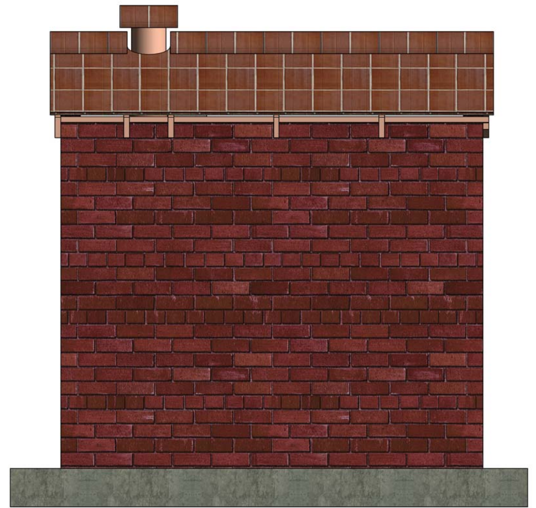
SIDE ELEVATION OF COMPLETE EXAMPLE VESUVIUS OVEN SCALE AT 1:20 ON A3
