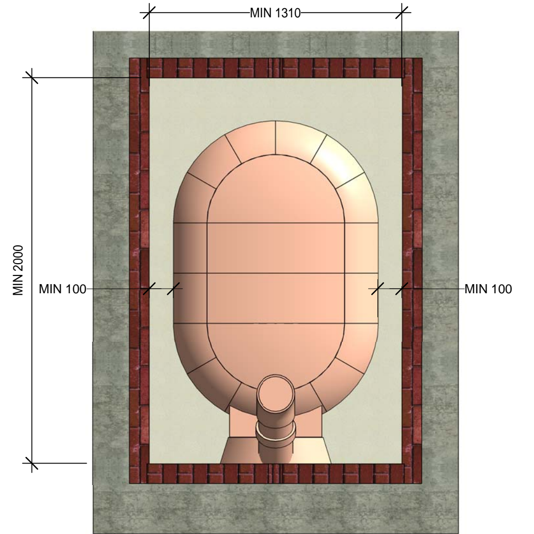
PLAN VIEW OF EXAMPLE VESUVIUS OVEN WITHOUT ROOF SCALE AT 1:20 ON A3
